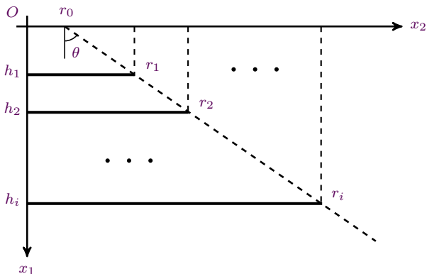
Geometric scheme for calculating the seismic efficiency
