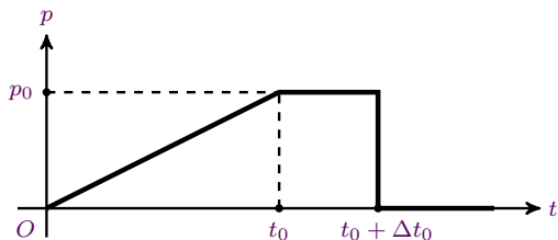
Graph of pressure from the source
