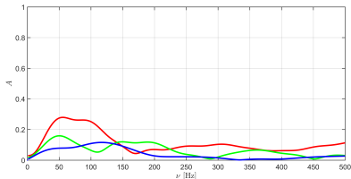
Amplitude-frequency dependences for velocity v_1 at the depth of 30 m
