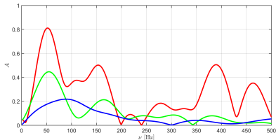
Upper layer is ice, middle layer is water
