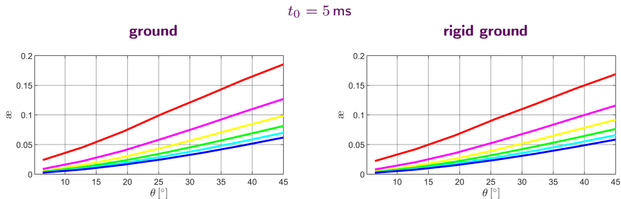
Dependences of the efficiency \alpha of a pulse seismic source on depth h_i and angle \theta for a ground and a rigid ground
