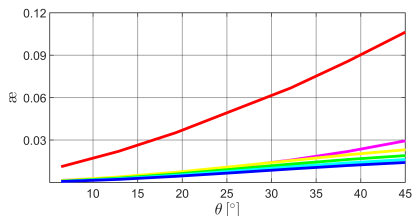
ice – water – ground
