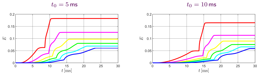
Dependences of the energy flux E_i on time in a ground
