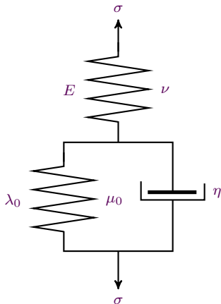
Rheological scheme of a viscoelastic material
