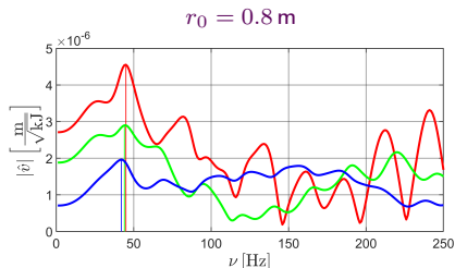
Amplitude–frequency characteristics of the velocity v_1 for a ground under static loading with instantaneous unloading
