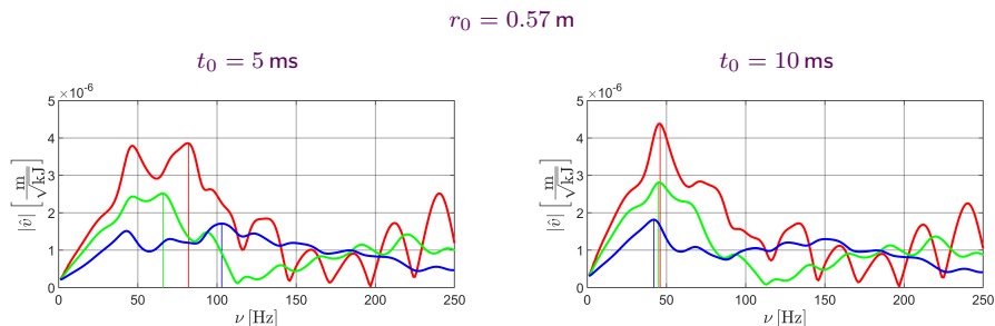
Amplitude–frequency characteristics of the velocity v_1 for a ground under dynamic loading
