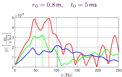
Amplitude–frequency characteristics of the velocity v_1 for a ground under dynamic loading
