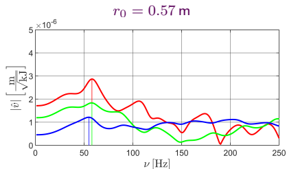
Amplitude–frequency characteristics of the velocity v_1 for a rigid ground under static loading with instantaneous unloading
